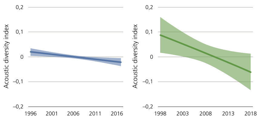
Changes in reconstructed soundscapes in North America (left) and Europe (right) over a period of 20 years
